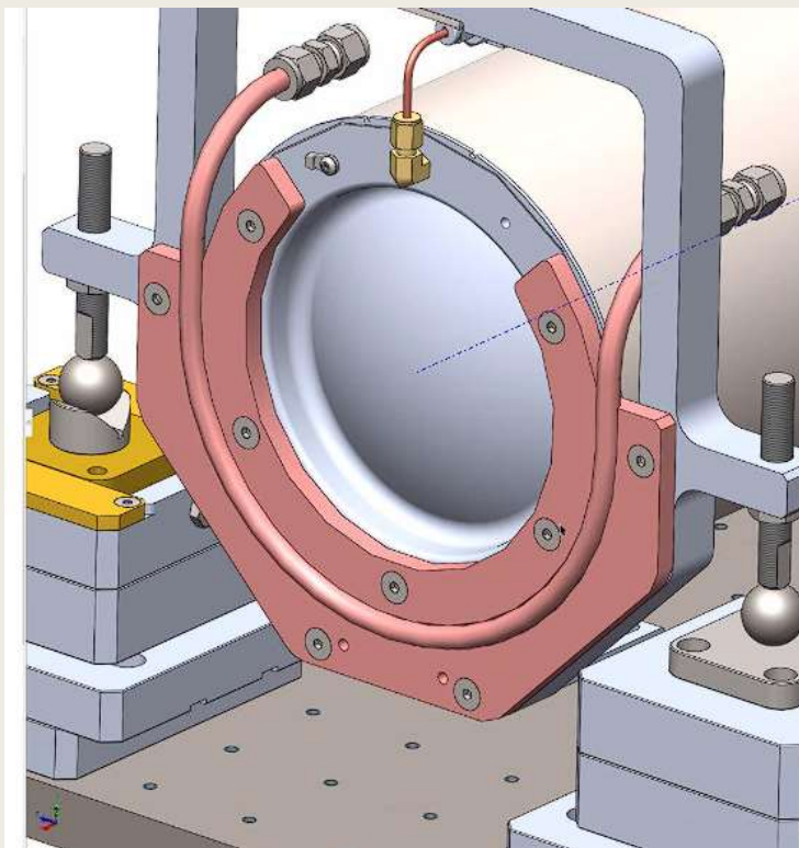
CAD Image
