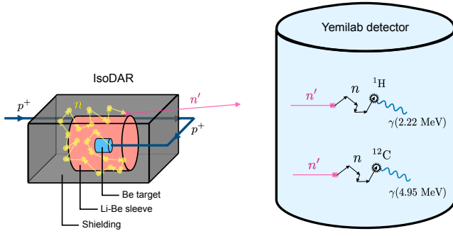
FIG. 1. The neutron-shining-through-a-wall signature at IsoDAR and the detection processes in the Yemilab liquid-scintillator detector [40, 41]. In the figure, we show the {}^7\text{Li} - {}^9\text{Be} -enriched sleeve enveloping the {}^9\text{Be} target. The sleeve is designed to increase the number of neutrons produced as well as their lifetime inside the sleeve [43], therefore also maximizing the number of n \rightarrow n' conversions. On the right we show two detection possibilities: neutron capture on H or C. Capture on Gd can also be considered, producing \sim 8 MeV photons.
