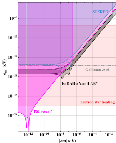
Figure: Plotted exclusion values and expected IsoDAR results.
