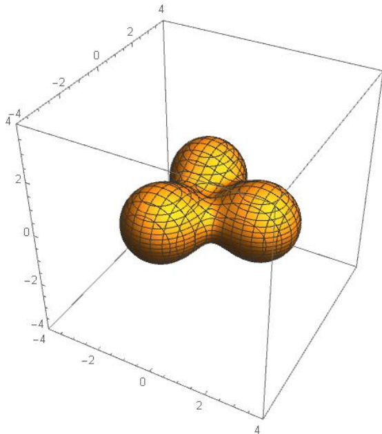
Ground state
