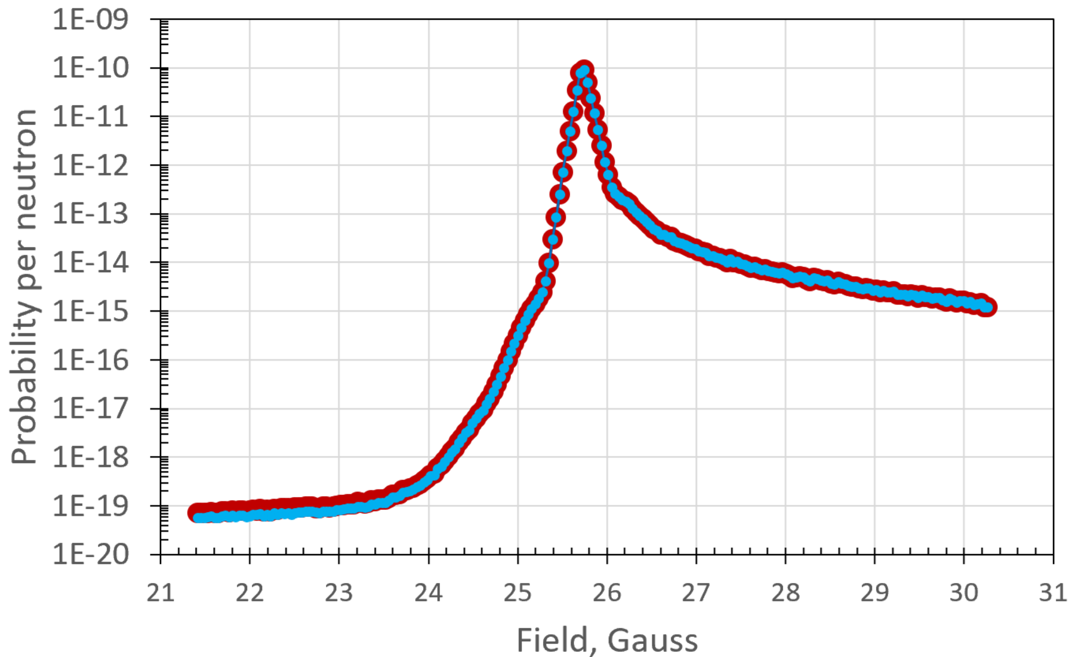
New Config with Poly (red) and wuthout Poly (blue)
