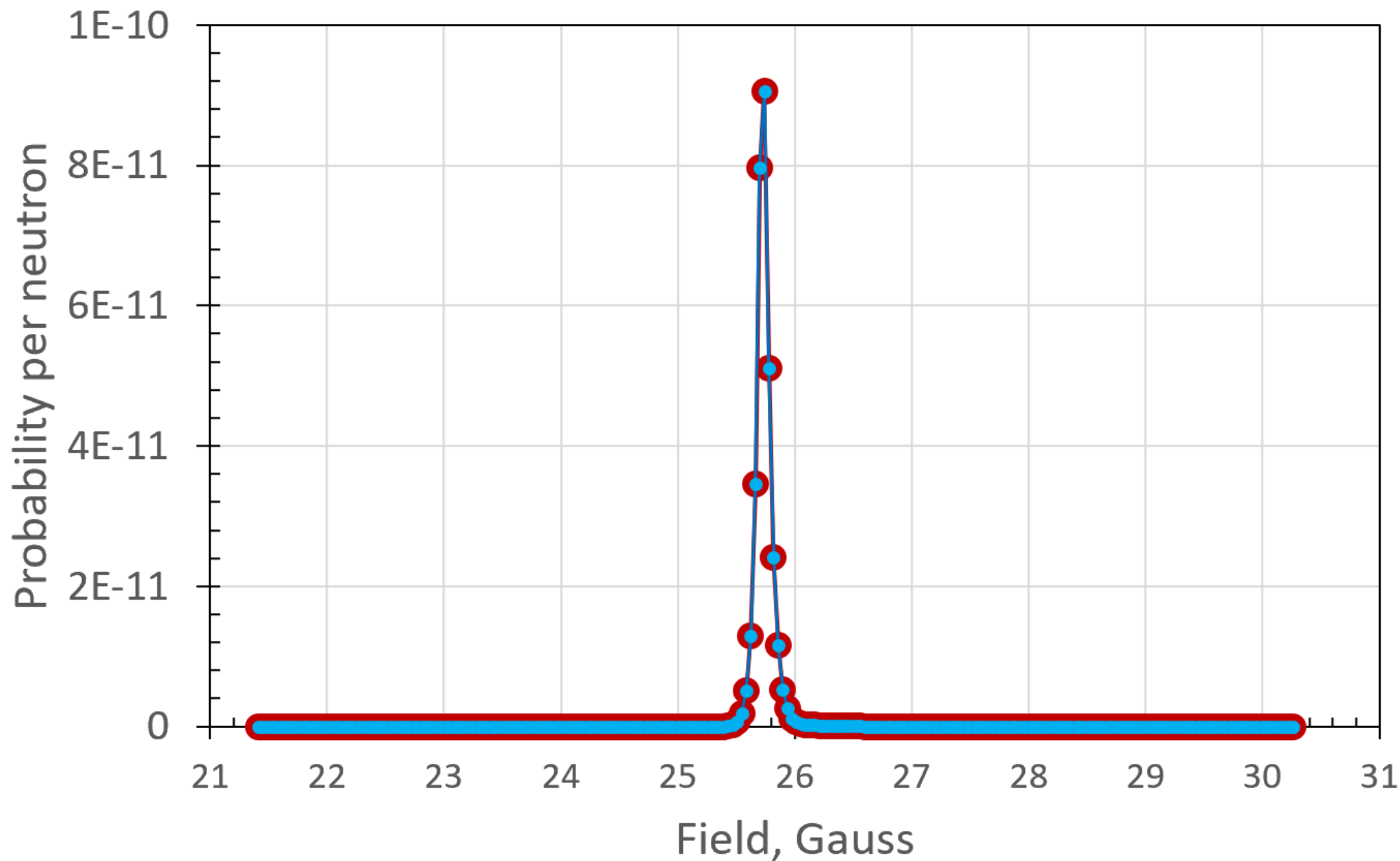
New Config with Poly (red) and without Poly (blue)
